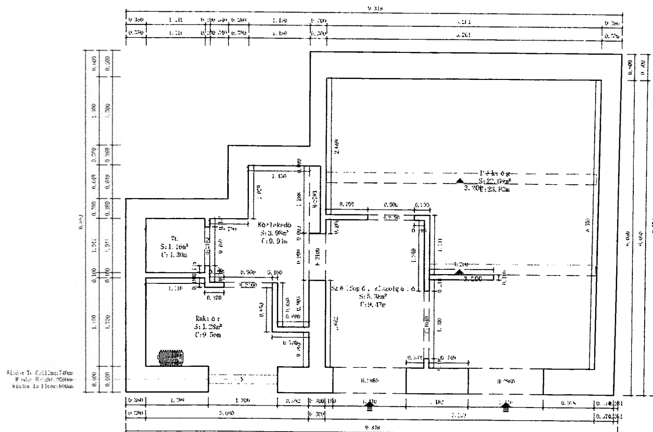
Floor Plan 1:50
