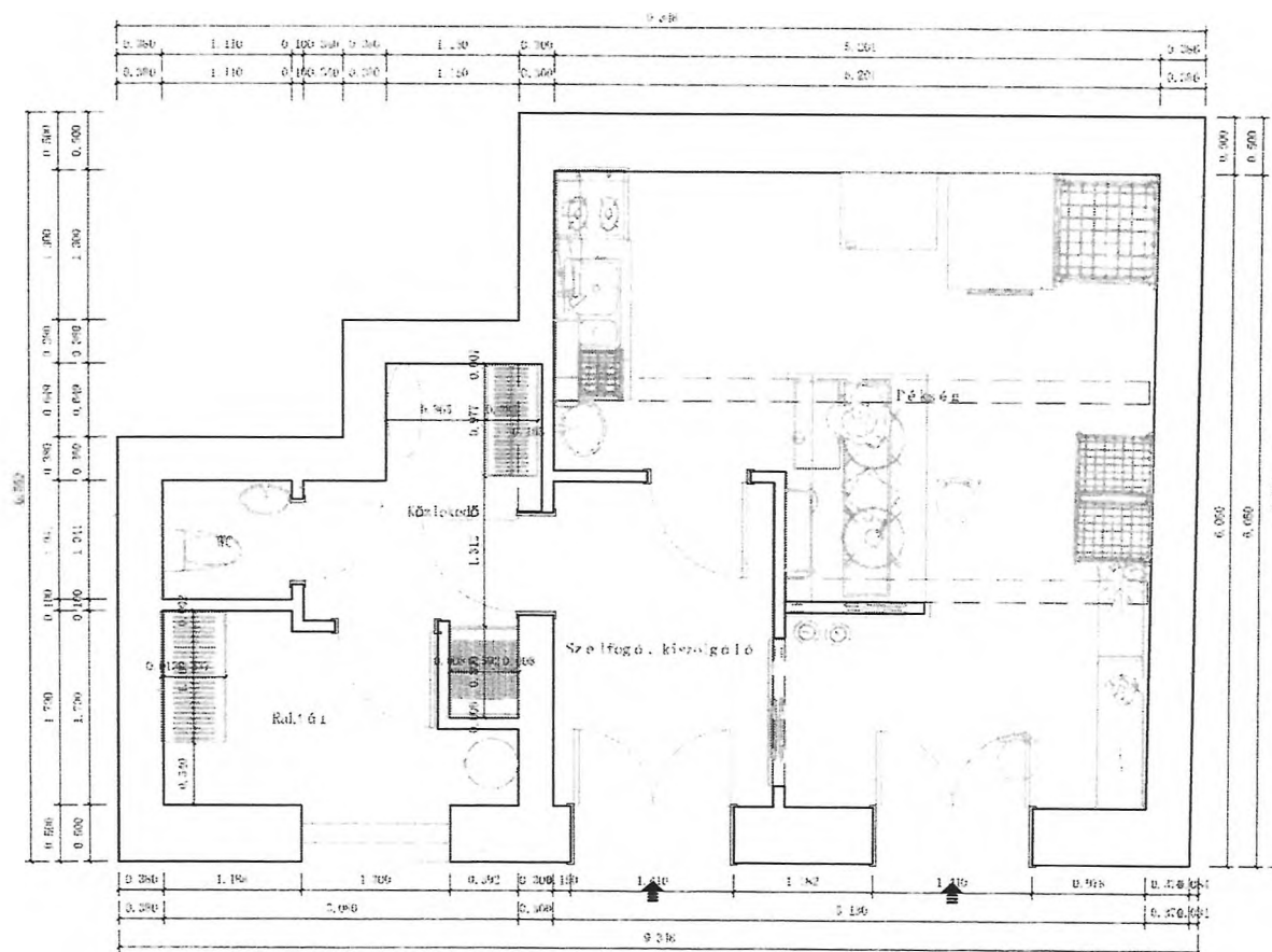
Furniture Size Plan 1:50
